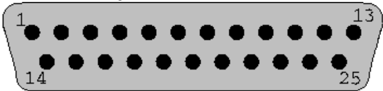
Figure 2 - RS-232 Connector
