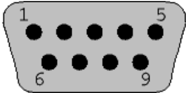
Figure 4 - RS-574 Connector
