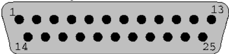
Figure 3 - RS-422 Connector
