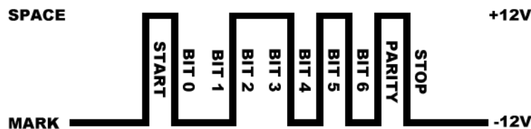
Figure 1 - Asynchronous Data Transmission
